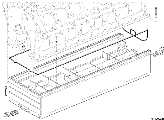
OIL PAN FLAT UPC.06E00 0825
